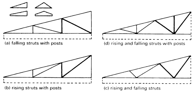
8 Timber construction forms and reinforcements
